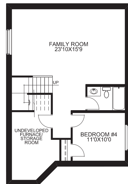
BASEMENT DEVELOPMENT PLAN 635 SQ.FT. DEVELOPED
