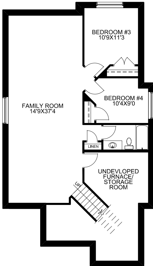
OPTIONAL LOWER DEVELOPMENT 937 SQ.FT. DEVELOPED
