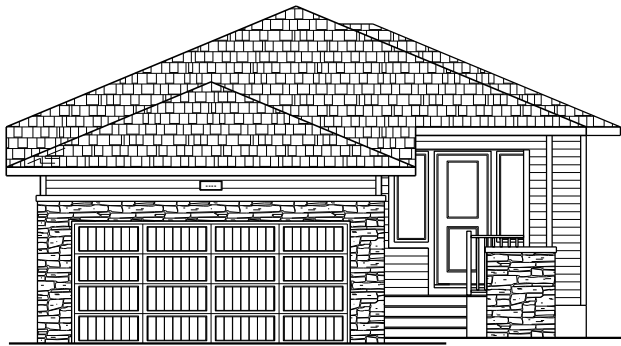
PRAIRIE ELEVATION
