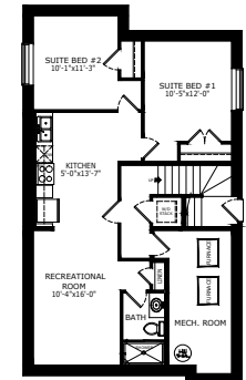
2 BEDROOM 'LEGAL SUITE' 816 SQ FT
